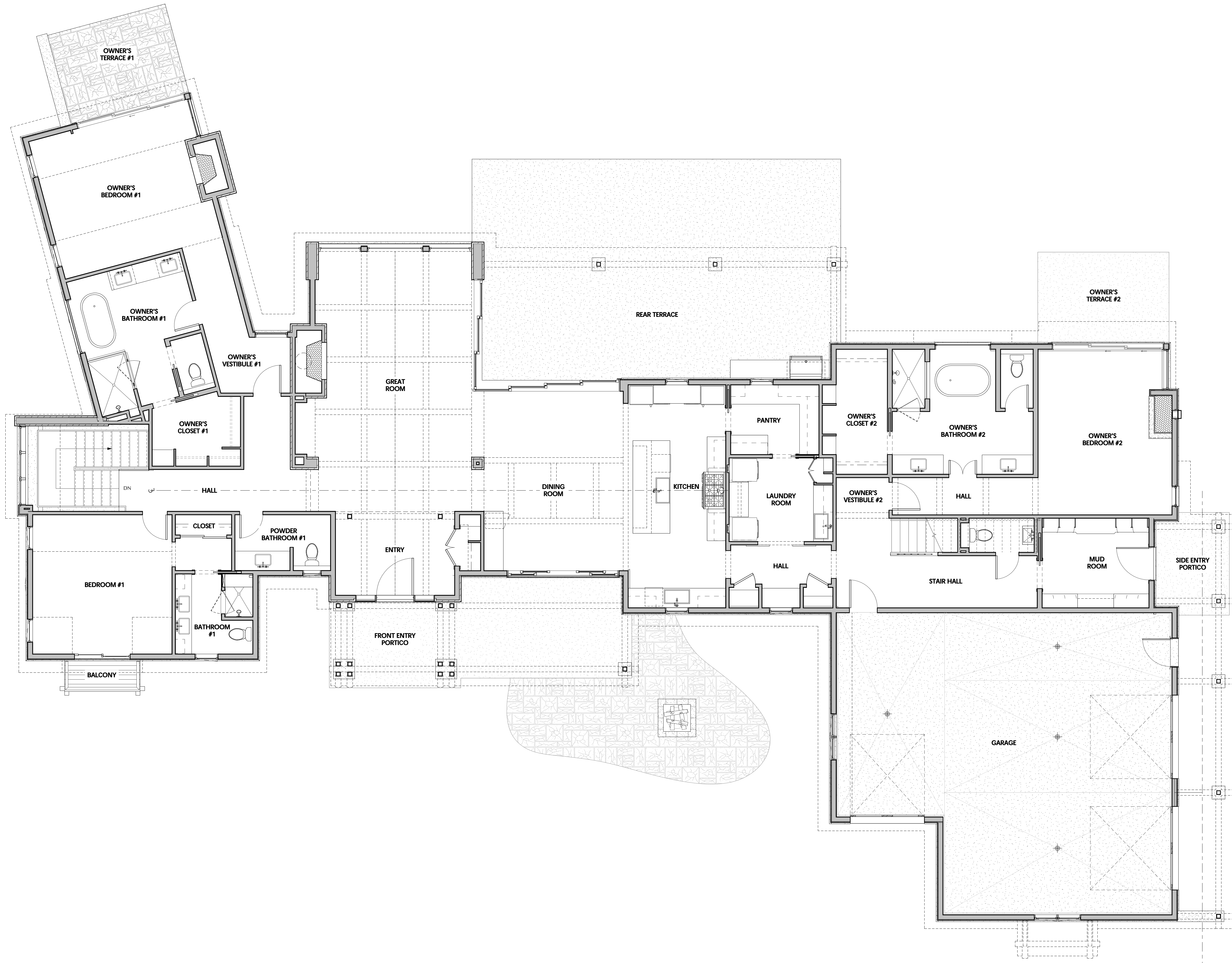
① FIRST FLOOR 1/4" = 1'-0"
